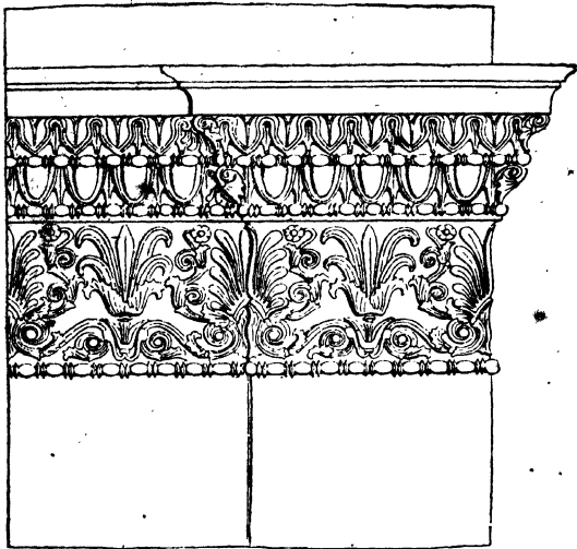
CORINTHIAN PILASTER.
